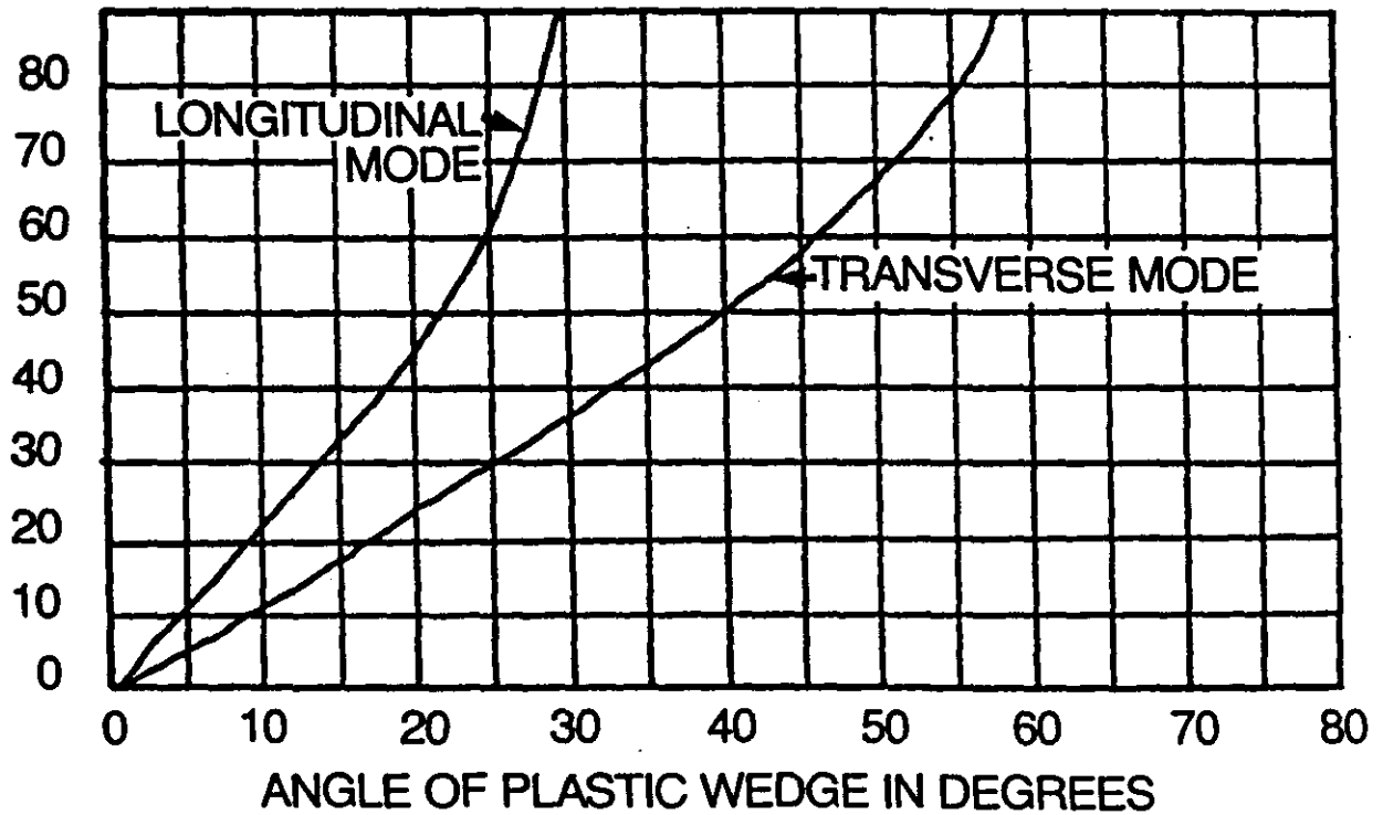
Figure 2.11: Longitudinal, Transverse and Surface Waves in a Wedge
