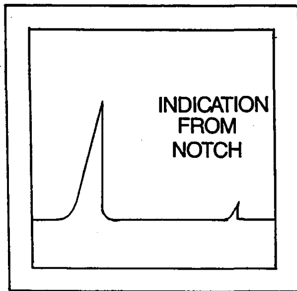
Figure 2.19: Pipe Inspection
