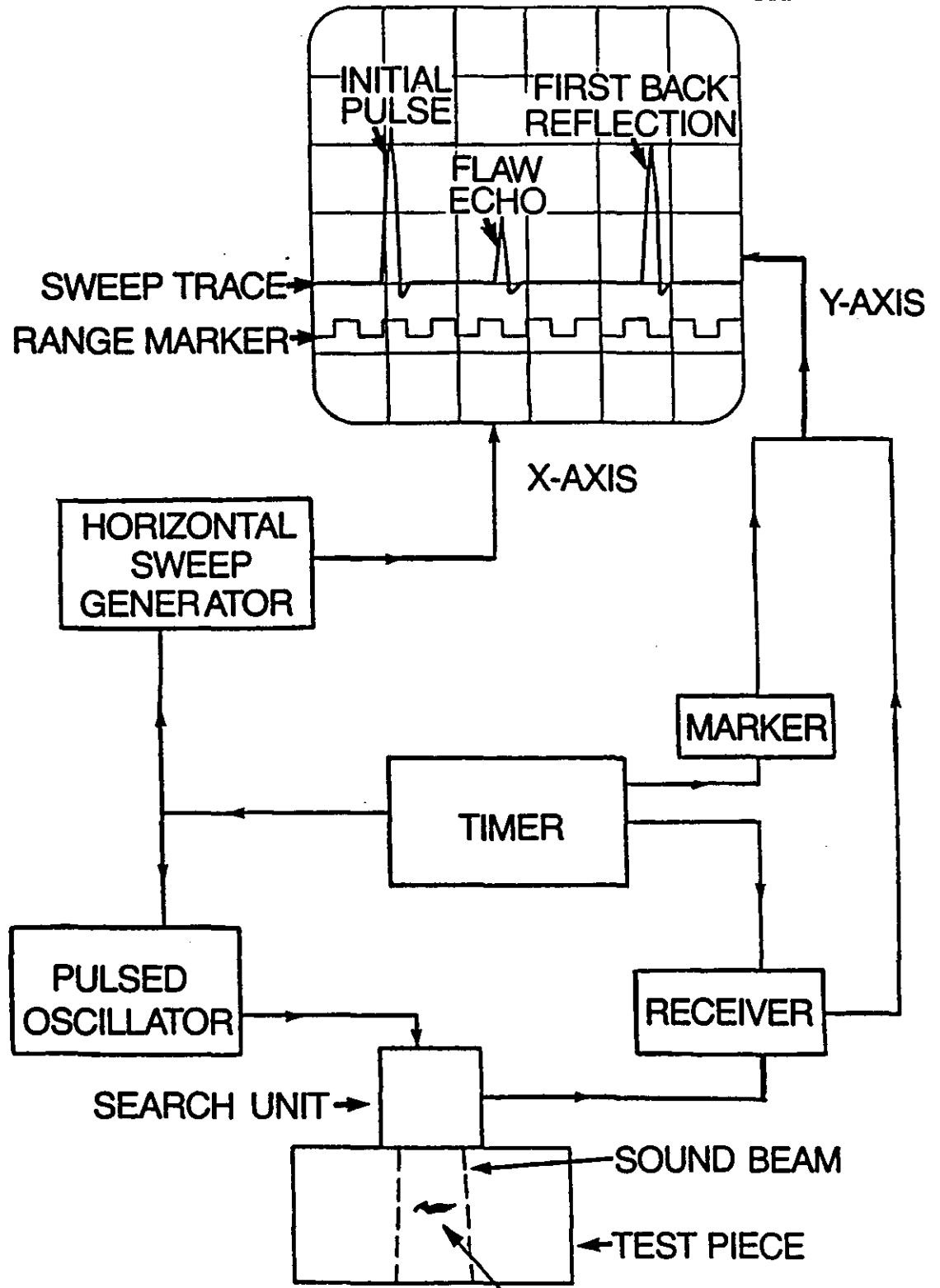
Figure 2.14: A-Scan FLAW
