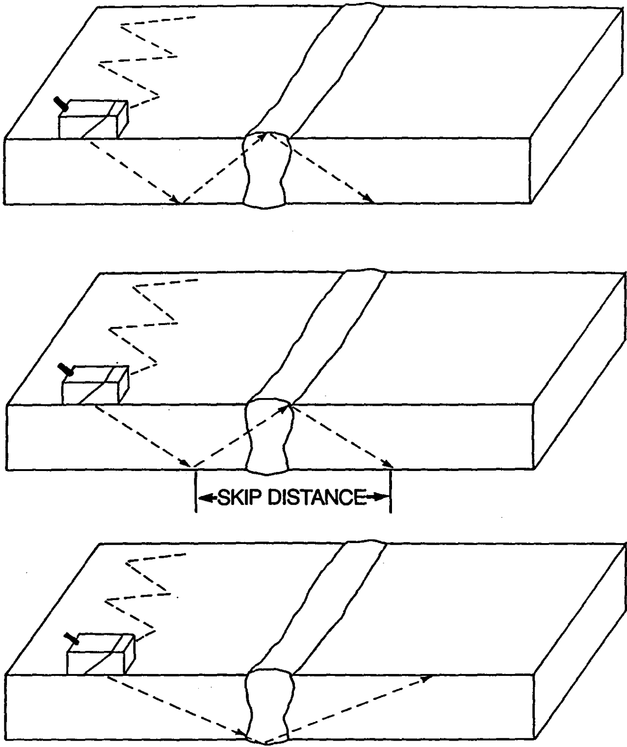
Figure 2.18: Weld Inspection with Node Technique
